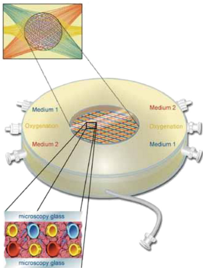
Fig. 8. Gerlach and co-workers developed a miniaturized hollow fiber perfusion design consisting of three fibers interwoven in two layers in an alternating fashion where hydrophilic membranes are employed for medium perfusion and hydrophobic membranes are employed for gas perfusion. This arrangement enables the reduction of bioreactor volume to 0.5 mL and subsequently the required number of cells [98].
