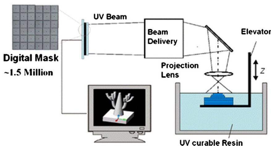
Fig. 14. A schematic showing the process of P \mu SLA, a recently developed technique for generating complex 3D micro-architecture tissue scaffolds with very high ( \sim 1\ \mu\text{m} ) feature resolution. Free-form fabrication techniques are likely going to prove applicable to the fabrication of scaffolds capable of guiding liver tissue morphogenesis and organization. The depicted technique is able to build structures similar to branching vasculature and biliary networks, and could prove a useful tool for future efforts to develop in vitro tissue analogs with histological architecture similar to that found in vivo [182].
