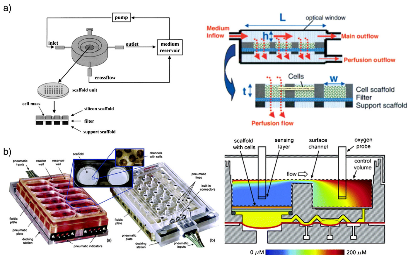
Fig. 13. Evolution of bioreactors for high-throughput 3D packed hepatocyte tissue culture. Original bioreactors (a) provided cross-flow perfusion, while also allowing through-tissue perfusion. Later reactors (b) allow the culture of up to twelve tissue constructs at a time, and are supported by a pneumatic platform that provides reliable control of flow through each tissue construct. Modeled oxygen concentrations for a perfused condition are shown in the right portion of (b) [139,138,147,156].
