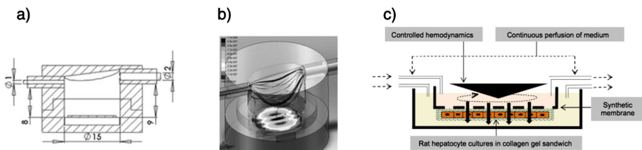
Fig. 3. (a) Multi-chamber Modular Bioreactor or McMB consists of a cell culture chamber made of PDMS and designed to accommodate the use of glass or plastic cover slips or scaffolds used for cell culture. (b) The McMB velocity profile showing stream lines. The McMB was designed with dimensions similar to a standard multiwell plate format, and operates in a low shear regime [66]. (c) A perfused transwell device using cone and plate technology with controlled hemodynamics mimics sinusoidal circulation. Hepatocytes cultured in a collagen gel sandwich configuration within the device exhibited polarized morphology and improvement of multiple hepatocellular functions relative to nonflow culture [68].
