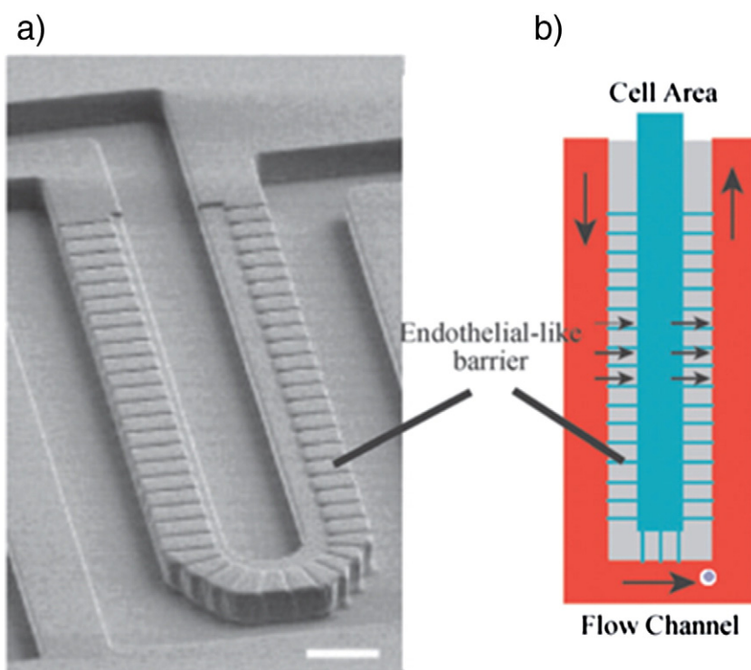
Fig. 11. A biologically inspired liver sinusoid with a microfluidic endothelial-like barrier developed by Lee and co-workers. (a) A SEM micrograph depicts the microfluidic sinusoid unit. (b) A cord of hepatocytes in the cell area region of the device is fed nutrients across the endothelial-like barrier via convective flow as media is fed through the outer flow channels. This device sustained rat and human hepatocytes for 7 days without the introduction of exogenous matrix [149].
