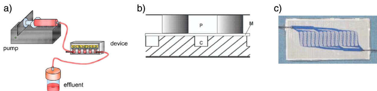
Fig. 5. (a) Bilayer PDMS device microfluidic setup with vascular and parenchymal compartments to mimic organ vasculature and support the metabolic demands of the liver cells. (b) Cross-sectional view of bilayer device showing the layers containing microfluidic channels (C), posts supporting the parenchymal chamber (P) and the intervening nanoporous polycarbonate membrane (M). (c) The assembled device was perfused with Trypan Blue through channels to demonstrate device integrity [75].
