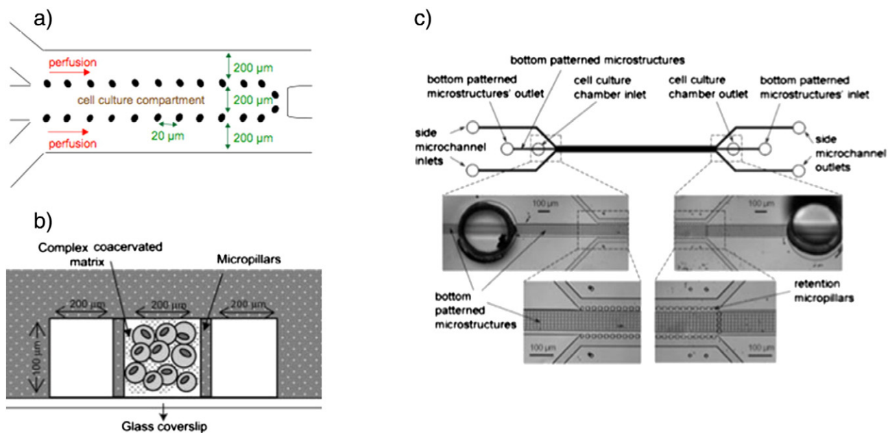
Fig. 12. (a) The gel-free 3D microfluidic channel-based cell culture system developed by Yu and coworkers. The microfluidic system has two inlets (one for culture medium infusion, one as cell reservoir) and one outlet. (b) Cross-sectional illustration of the same system. (c) Representation of another system developed by Goral et al. at Corning Incorporated to create 3D dynamic primary human hepatocyte cell culture without the addition of biological or synthetic matrices. [151,155,158].
